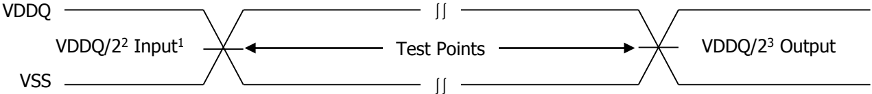
Figure 8. AC Input/Output Reference Waveform
