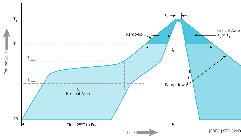
Figure 18. Visualization of the acceptable reflow temperature profile as specified in Table 10.
