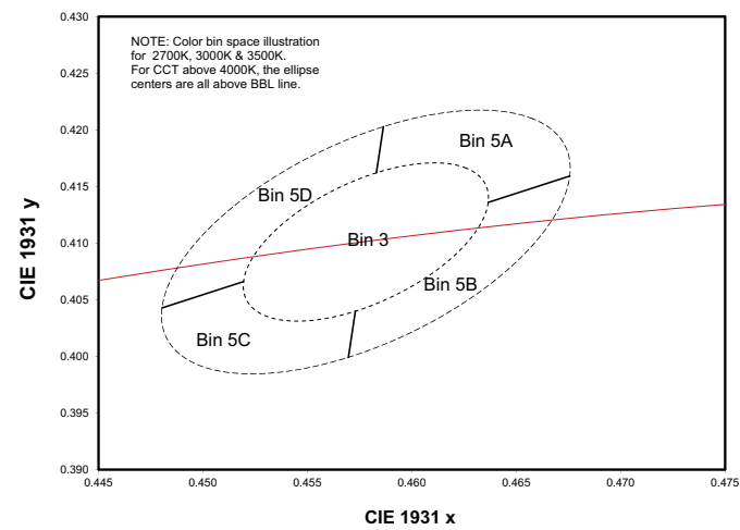
Figure 15. Color space definition for LUXEON HL2Z.
