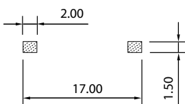
Lead design 1
