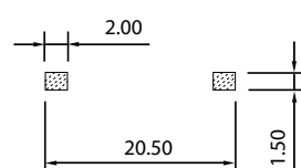
Lead design 4
