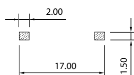
Lead design 2
