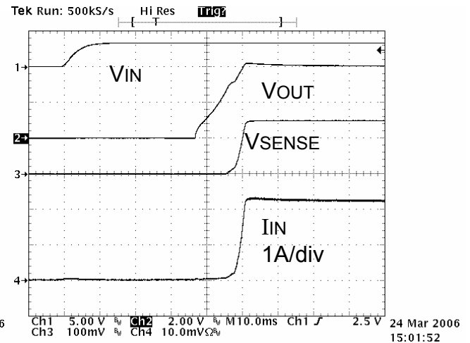
Start up VIN=3.3V
