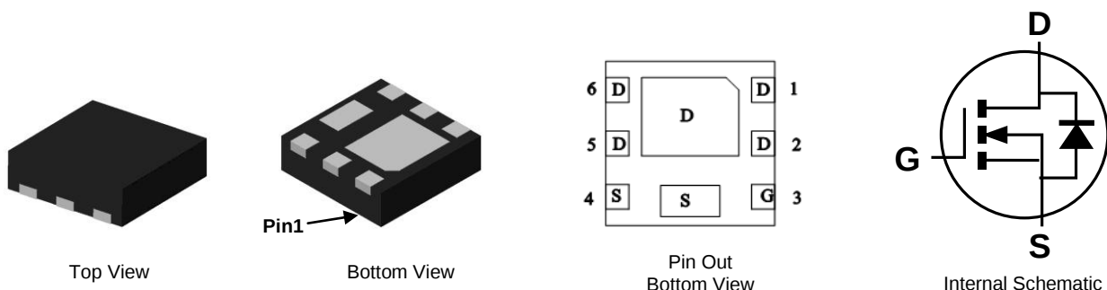
U-DFN2020-6 (Type F)
