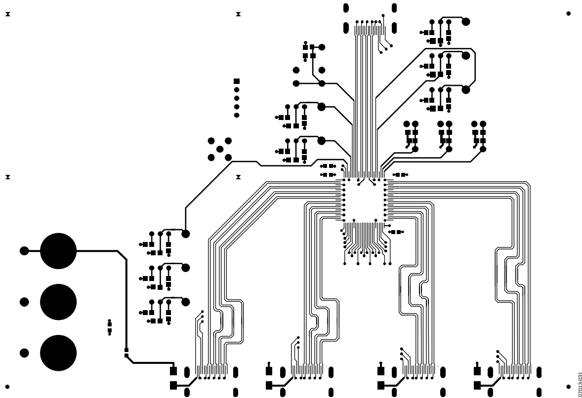
Figure 31. Layout of the TMDS Traces on the AD8191A Evaluation Board (Only Top Signal Routing Layer is Shown)
