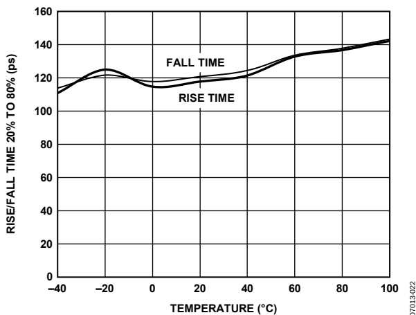
Figure 22. Rise/Fall Time vs. Temperature
