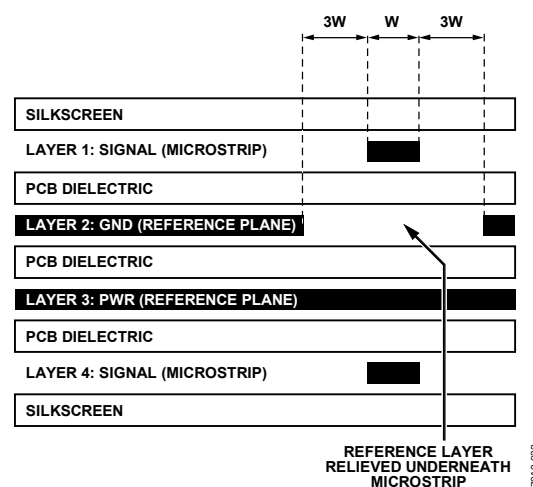
Figure 33. Example Board Stackup
