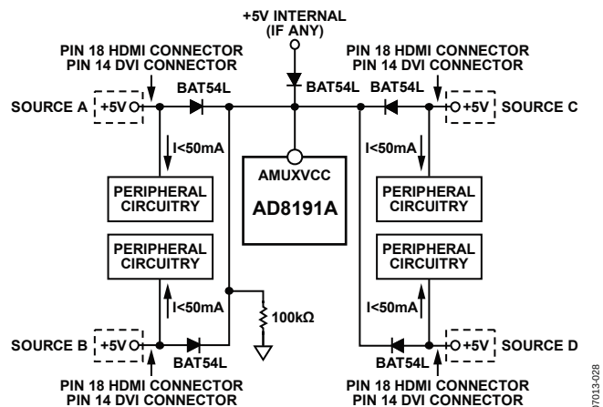
Figure 28. Suggested AMUXVCC Power Scheme
