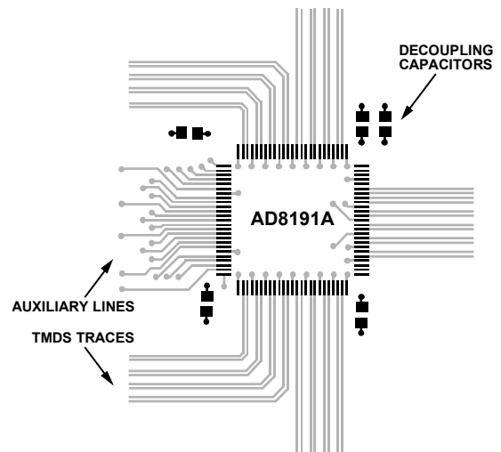
Figure 35. Example Placement of Power Supply Decoupling Capacitors Around the AD8191A
