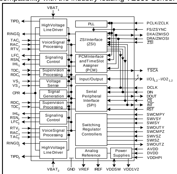
VoicePort Device Block Diagram
