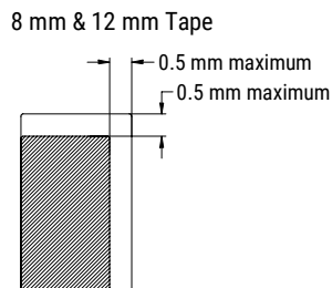
Figure 3 – Maximum Lateral Movement
