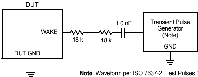
Figure 5. Test Circuit for Transient Test Pulses (WAKE)
