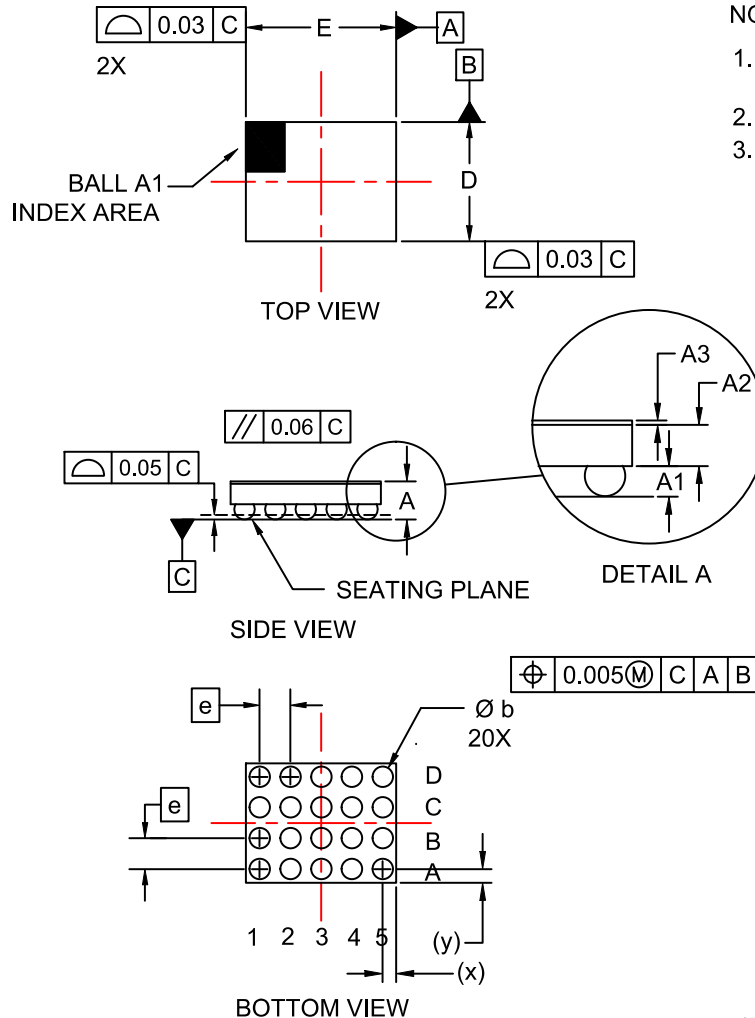
WLCSP20 1.61x1.96x0.432 CASE 567YA ISSUE O
