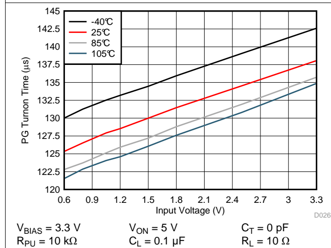
Figure 21. PG Turnon Time vs Input Voltage
