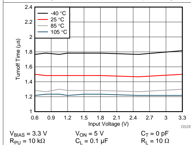
Figure 23. PG Turnoff Time vs Input Voltage
