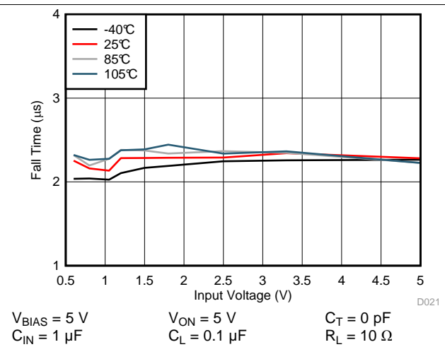
Figure 20. Fall Time vs Input Voltage
