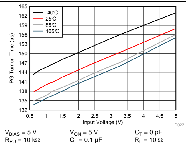
Figure 22. PG Turnon Time vs Input Voltage
