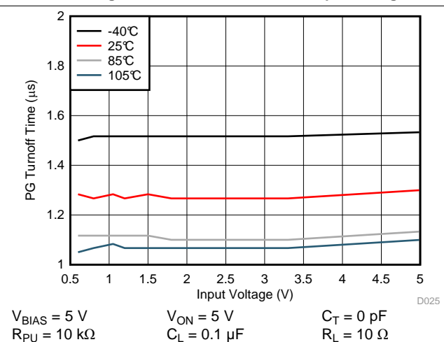
Figure 24. PG Turnoff Time vs Input Voltage
