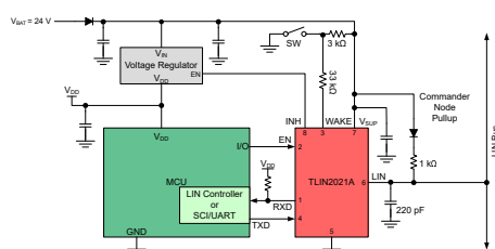
Simplified Commander Node Schematic
