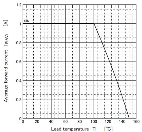
Derating curve
