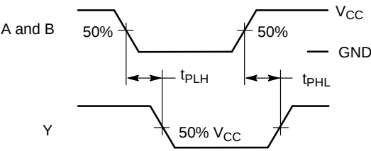
PROPAGATION DELAYS t_R = t_F = 2.5 \text{ ns} , 10% to 90%; f = 1 \text{ MHz} ; t_W = 500 \text{ ns}
