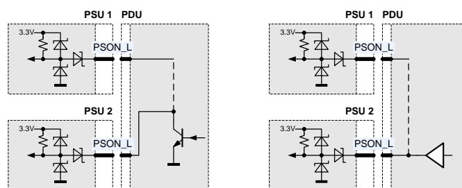
Figure 18. PSON_L connection
