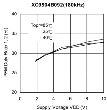
(23) PFM Duty Ratio1, 2 vs. Supply Voltage
