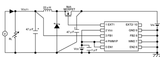
Circuit 4
