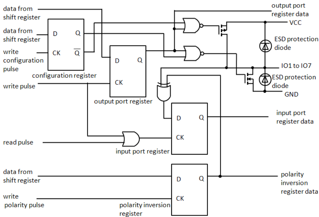
Figure 5: Simplified schematic of IO1 to IO7
