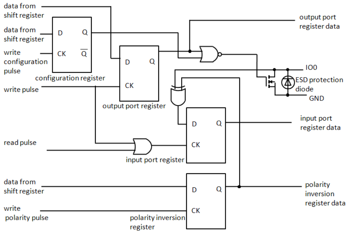
Figure 4: Simplified schematic of IO0
