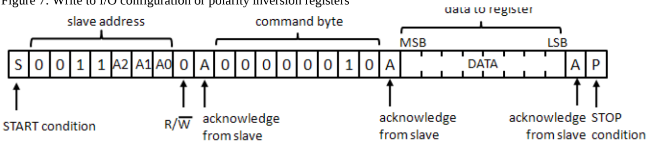
Figure 7: Write to I/O configuration or polarity inversion registers
