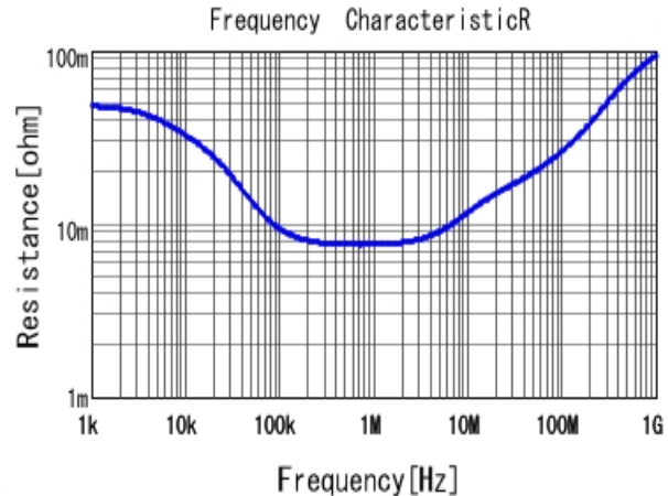
■ ECASD40J476M025K00 R DC0V, 25degC
