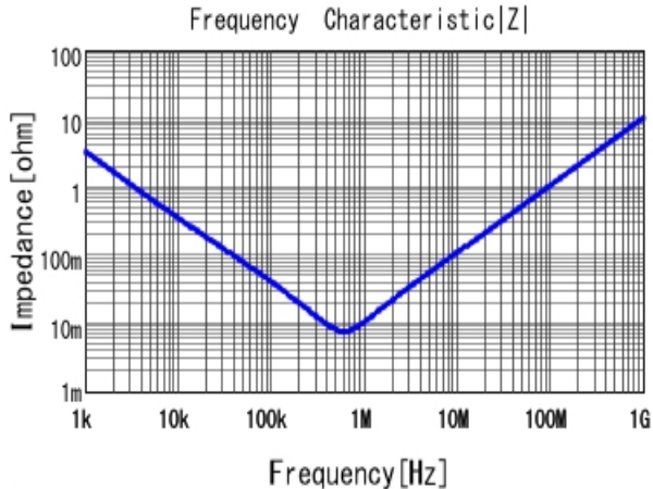
■ ECASD40J476M025K00 |Z| DC0V, 25degC
