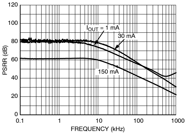
Figure 27. PSRR, 0.8 V Version, V_{IN} = 1.8\text{ V}
