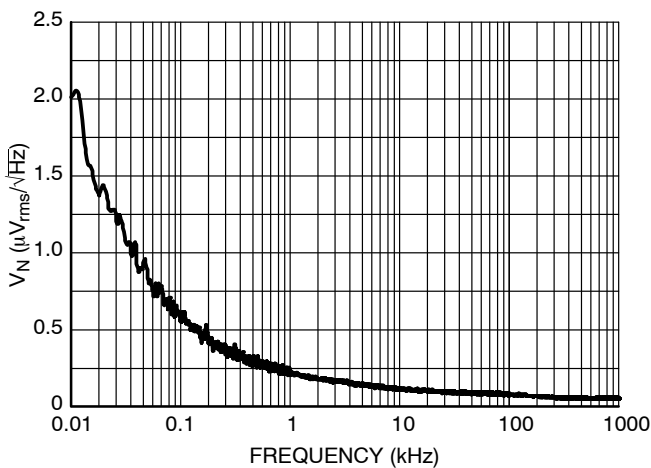
Figure 31. Output Voltage Noise, 0.8 V Version, V_{IN} = 1.8\text{ V}
