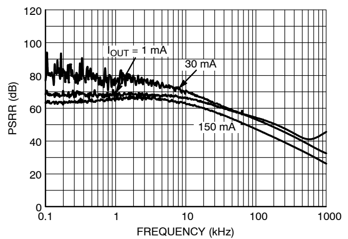
Figure 30. PSRR, 3.3 V Version, V_{IN} = 4.3\text{ V}
