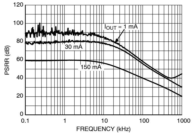
Figure 28. PSRR, 1.8 V Version, V_{IN} = 2.8\text{ V}
