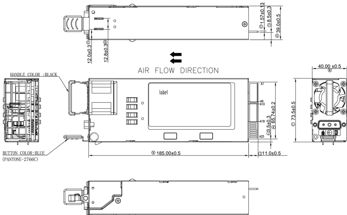
Figure 5. Mechanical Drawing
