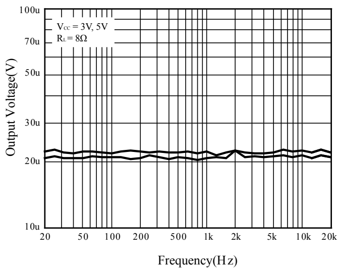
Figure 7 Noise Floor
