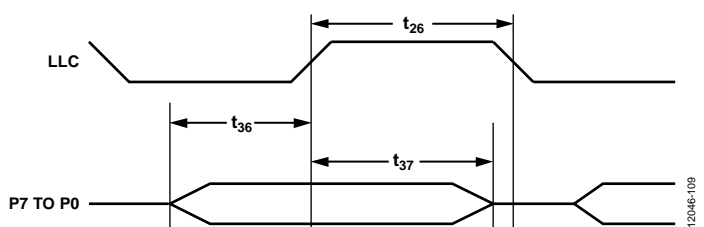
Figure 8. 8-Bit Digital Pixel Video Input, DDR Video Data Timing
