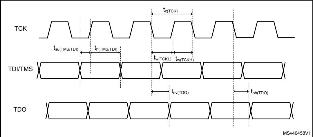
Figure 58. JTAG timing diagram
