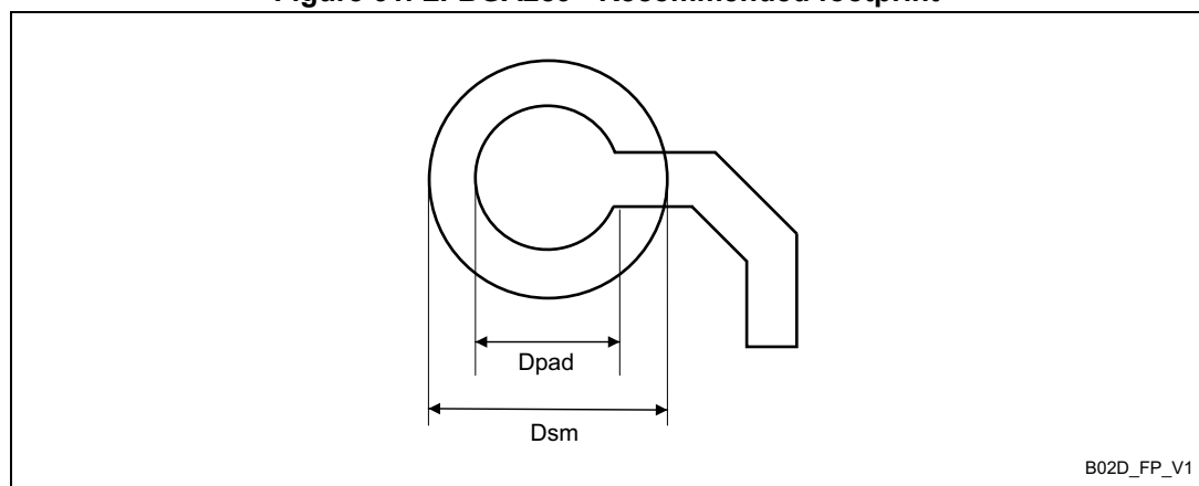
Figure 61. LFBGA289 - Recommended footprint
