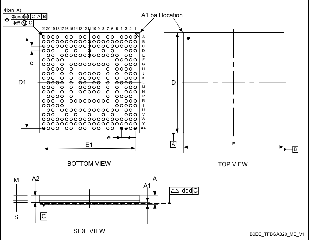
Figure 64. TFBGA320 - Outline
