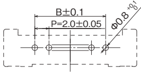
Recommended PCB Layout (t=1.6mm)
