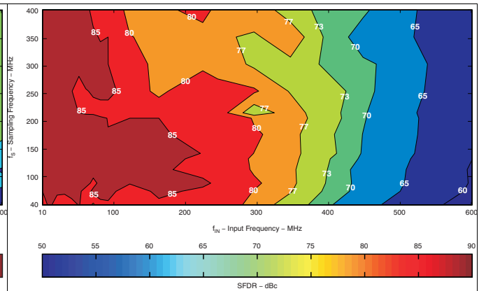
Figure 33. SFDR vs Input Frequency And Sampling Frequency
