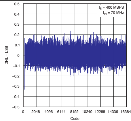
Figure 15. Differential Nonlinearity
