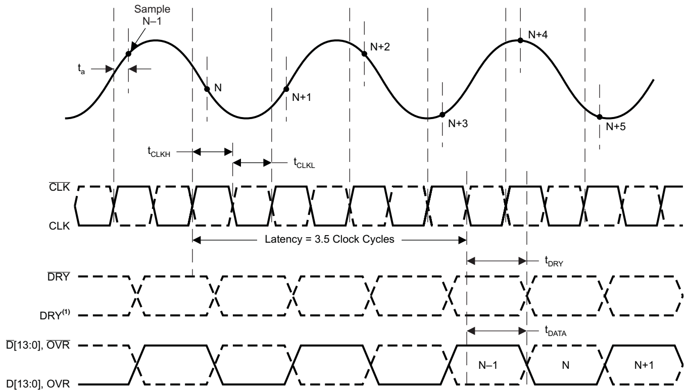
Figure 1. Timing Diagram
