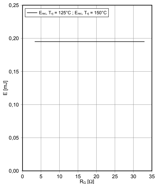
Schaltverluste Diode, 3-Level (typisch) switching losses Diode, 3-Level (typical) E_{rec} = f(R_G) I_F = 60 \text{ A} , V_{CE} = 600 \text{ V}
