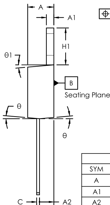
TO220-2 10.16x15.37x4.19, 5.08P CASE 340AZ ISSUE B
