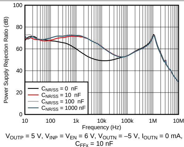
Figure 10. Positive PSRR vs Frequency and C_{\text{NR/SS}}
