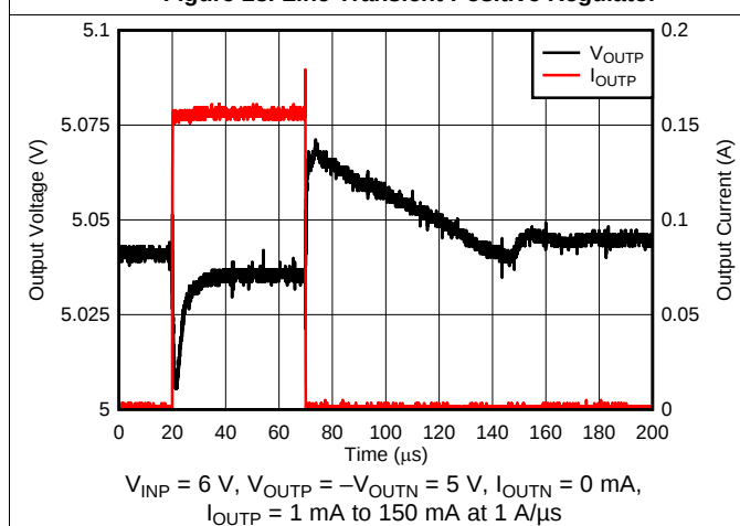
Figure 30. Load Transient Positive Regulator
