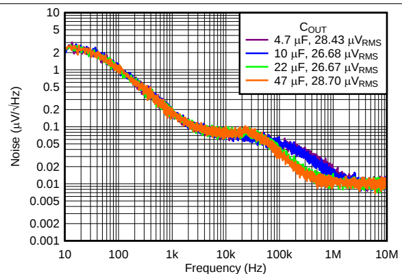
Figure 21. Negative Spectral Noise Density vs Frequency and C_{\text{OUT}}
