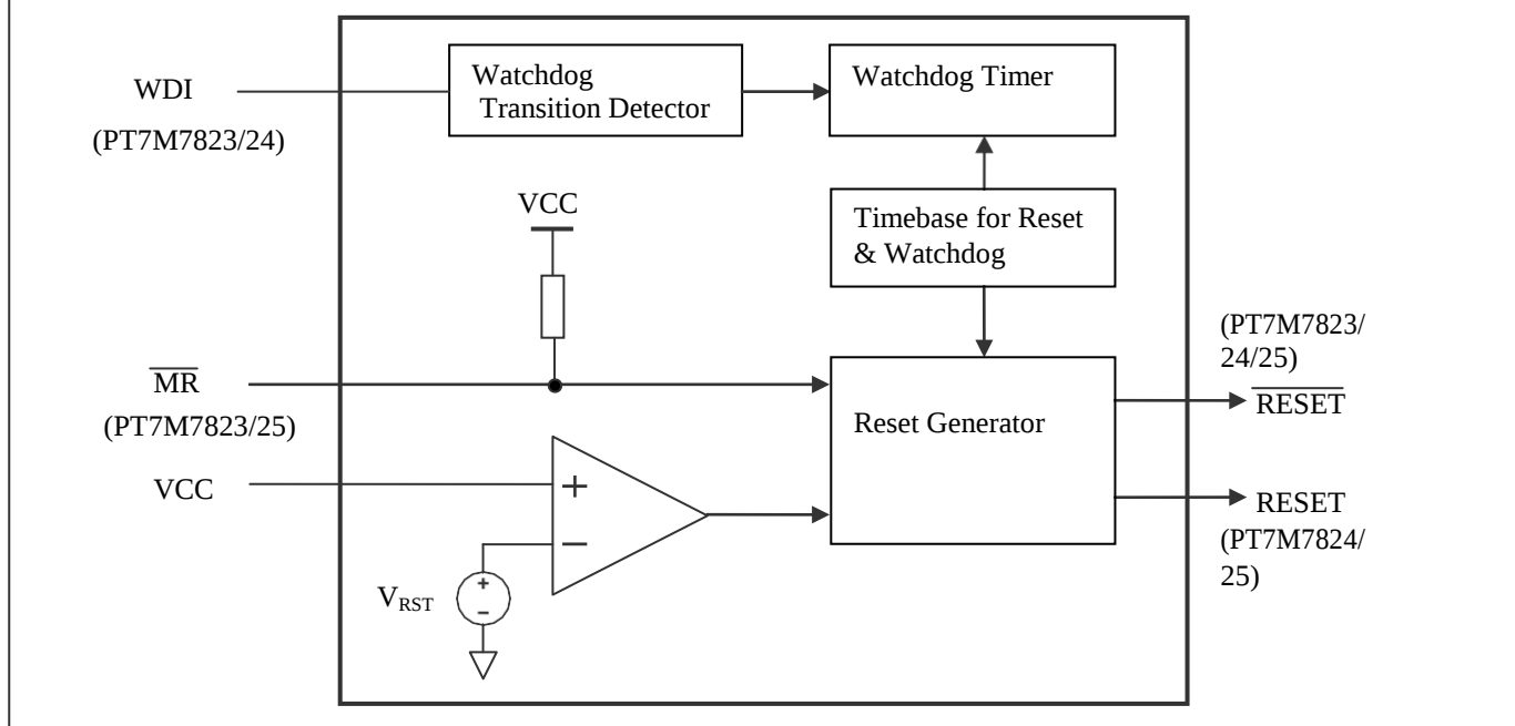
PT7M7823/24/25 Block Diagram
