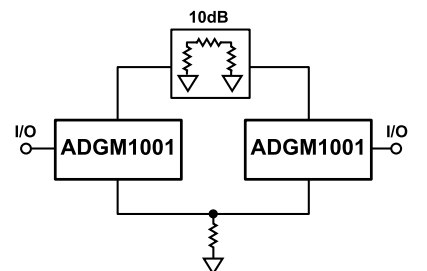
Figure 59. Switching RF Attenuators Using ADGM1001 MEMS Switches
