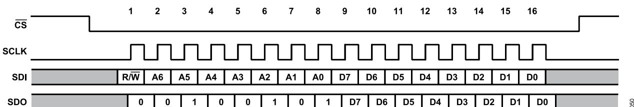
Figure 52. Addressable Mode Timing Diagram (Mode 0)
