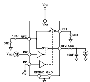
Figure 67. DC Hot Switching Setup
