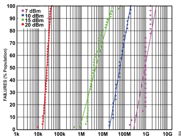
Figure 66. RF Hot Switching Probability Distribution on Log Normal (RF Power = Continuous Wave, Terminated into 50 \Omega , T_A = 25^\circ\text{C} , V_{DD} = 3.3\text{ V} )
