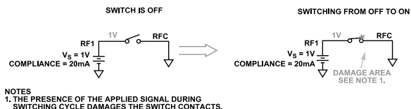
Figure 63. Hot Switching Condition When Turning the Switch from Off to On State
