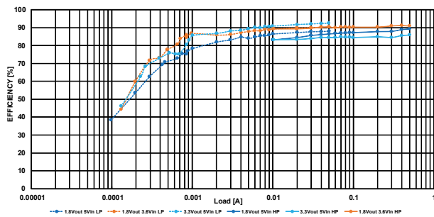
Figure 5. BUCK3 efficiency
