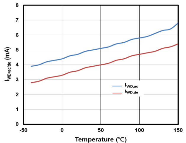
Figure 16. Watchdog Activation/Deactivation Current vs. Junction Temperature
