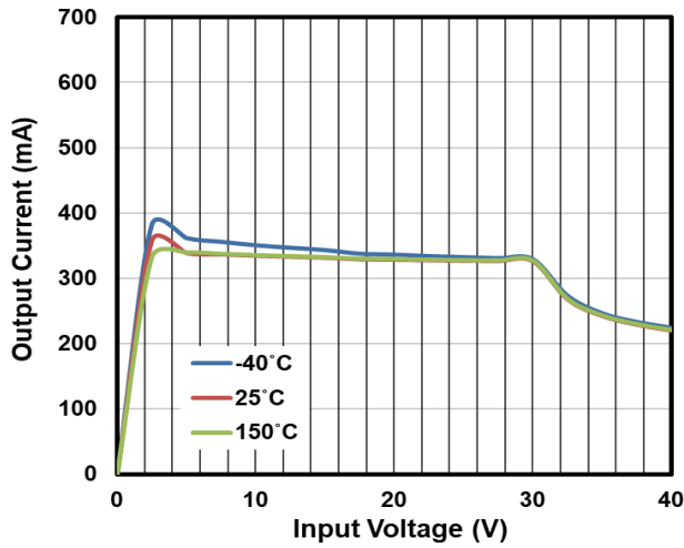
Figure 7. Output Current vs. Input Voltage
