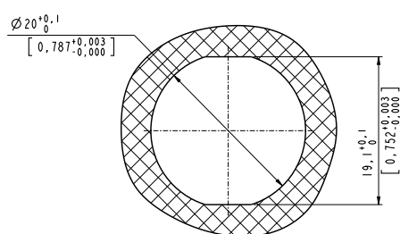
Panel rilling
