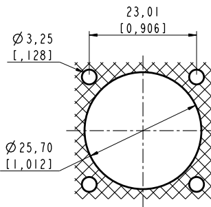
Panel drilling
