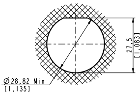
Panel drilling
