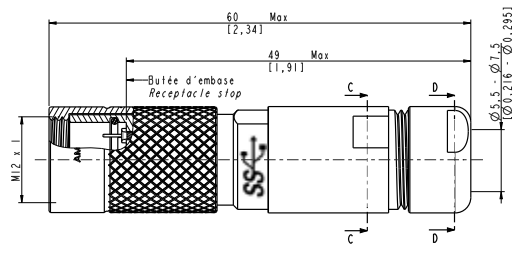
Thread version
