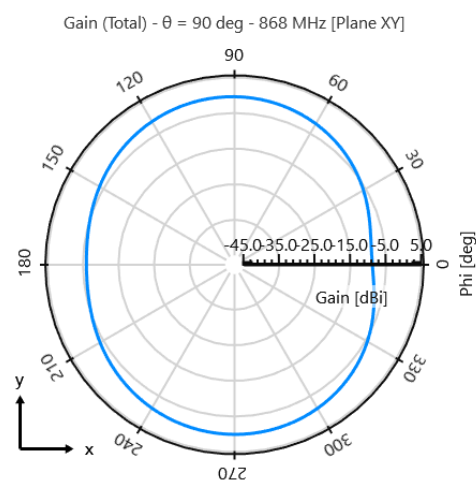
Theta = 90° Plane
