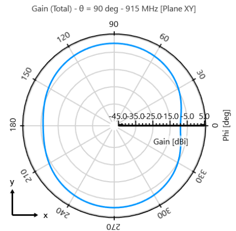
Theta = 90° Plane
