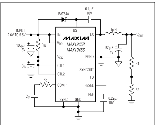
Figure 2. Typical Application Circuit (Adjustable Output Voltage)
