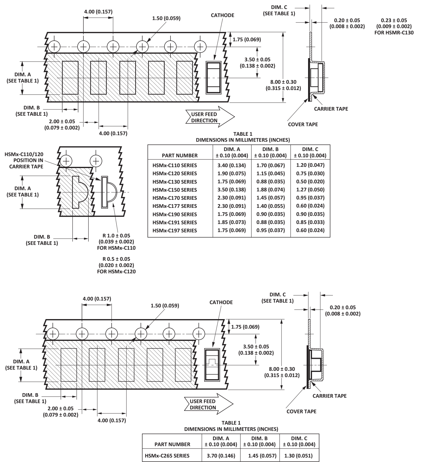
Figure 23: Tape Dimensions
