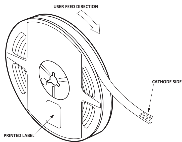
Figure 21: Reeling Orientation
