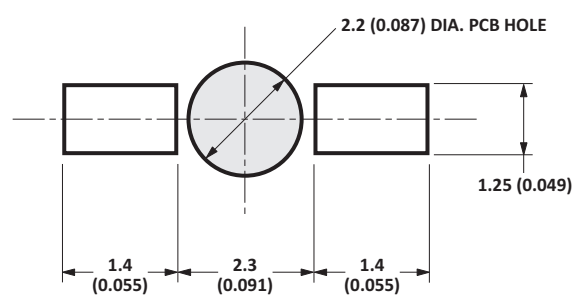
Figure 20: Recommended Soldering Pattern for HSMx-C265
