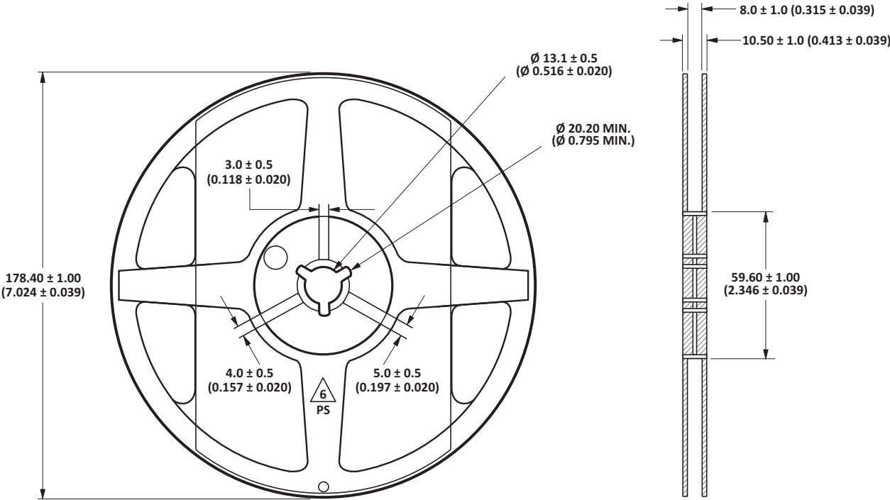
Figure 22: Reel Dimensions
