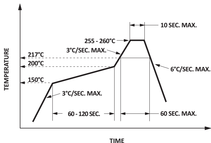
Figure 14: Recommended Pb-free Reflow Soldering Profile
