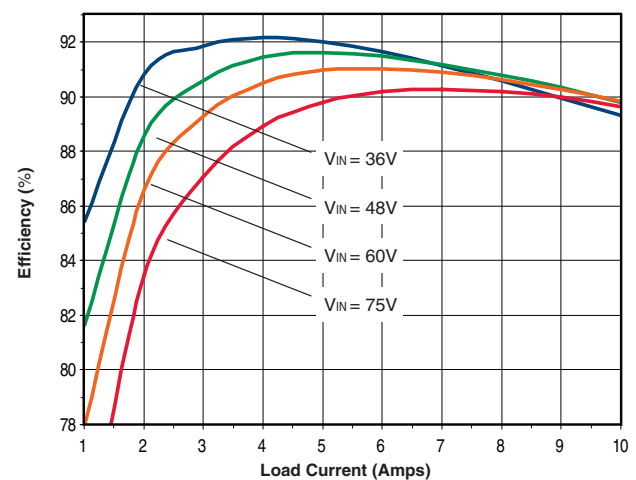
UVQ-12/10-D48N Efficiency vs. Line Voltage and Load Current @ +25°C
