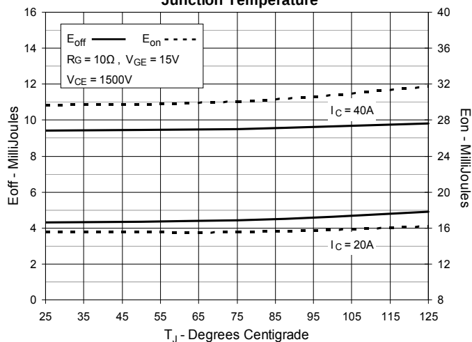
Fig. 17. Inductive Switching Energy Loss vs. Junction Temperature
