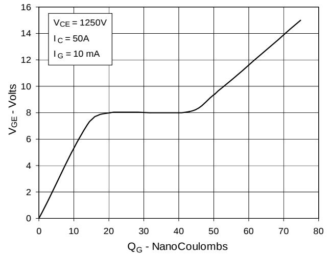
Fig. 14. Gate Charge
