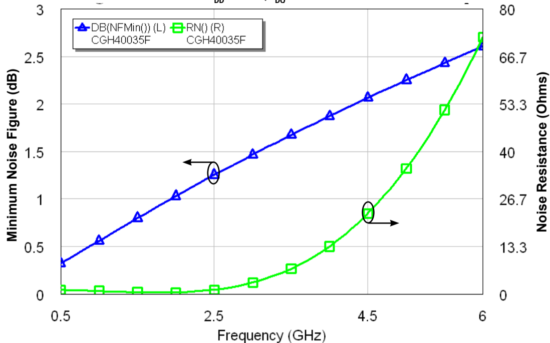
Simulated Minimum Noise Figure and Noise Resistance vs Frequency of the CGH40035F
