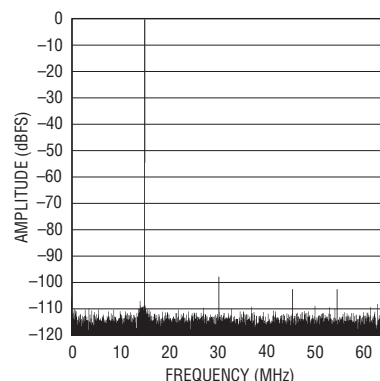
32k Point FFT, f_{IN} = 15.11\text{MHz} , -1dB, PGA = 0, RAND "On", Dither "OFF"
