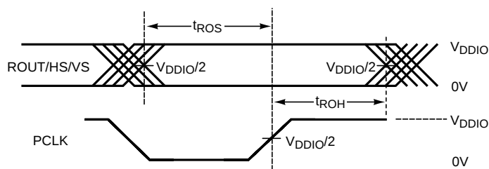
Figure 20. Deserializer Output Setup/Hold Times
