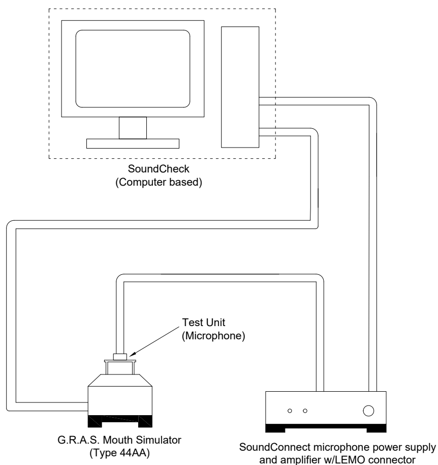
Figure 6. Test Setup
