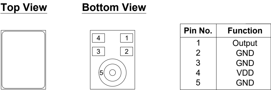
Figure 4. Electrical Layout of SMO08C-38/1086
