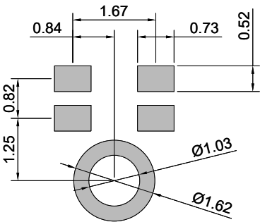
Figure 9. PCB solder pad layout for SMO08C-38/1086
