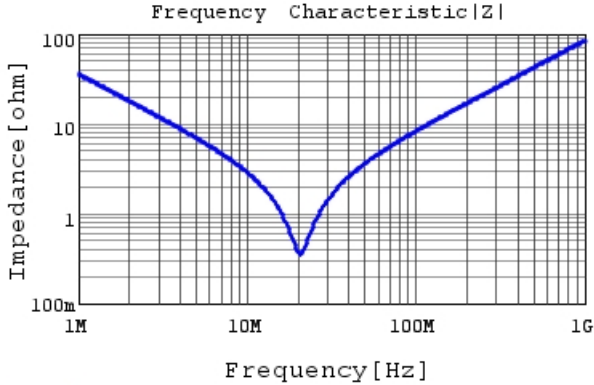
DE1E3RA472MN4AN01F |Z| DCOV, 20degC
