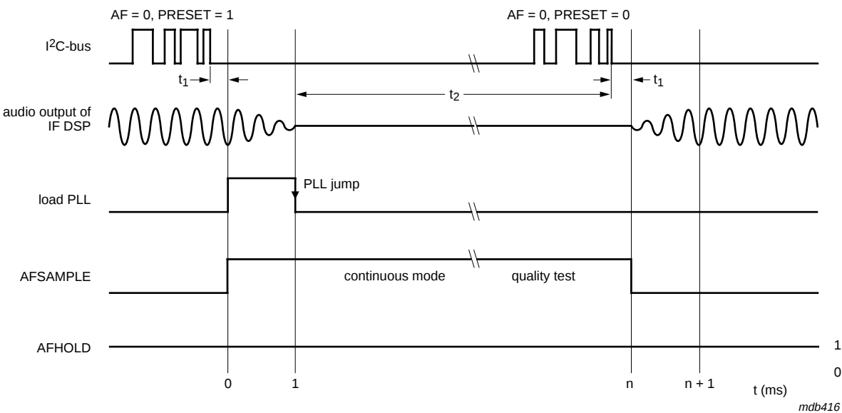
t_1 is the internal TEF6721HL clock related logic delay: 100 \mu s. t_2 should be greater than the required PLL tuning time for the given band (FM: t_2 > 1 ms; AM: t_2 > 20 ms).
