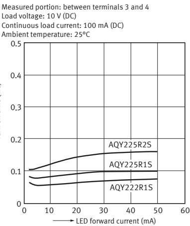
11. Turn off time vs. LED forward current characteristics
