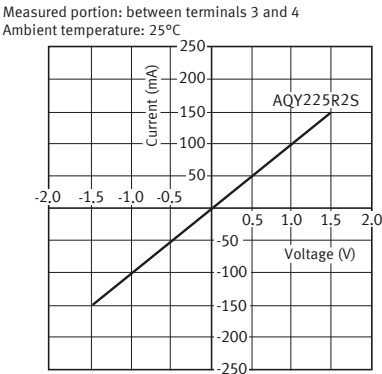
8-3. Current vs. voltage characteristics of output at MOS portion
