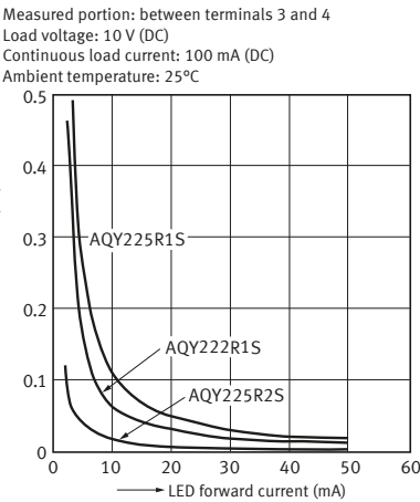
10. Turn on time vs. LED forward current characteristics
