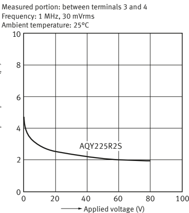
12-2. Output capacitance vs. applied voltage characteristics
