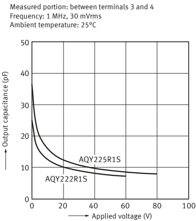
12-1. Output capacitance vs. applied voltage characteristics
