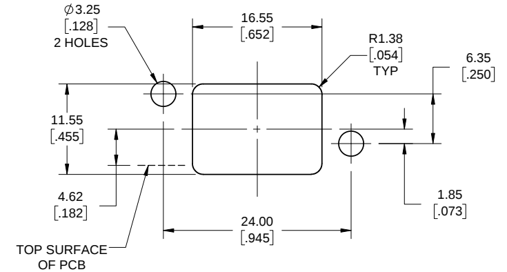
RECOMMENDED PANEL CUTOUT OUTSIDE VIEW OF PANEL
