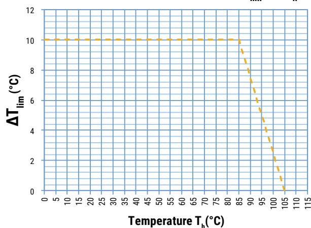
Maximum Overtemperature \Delta T_{lim} vs T h
