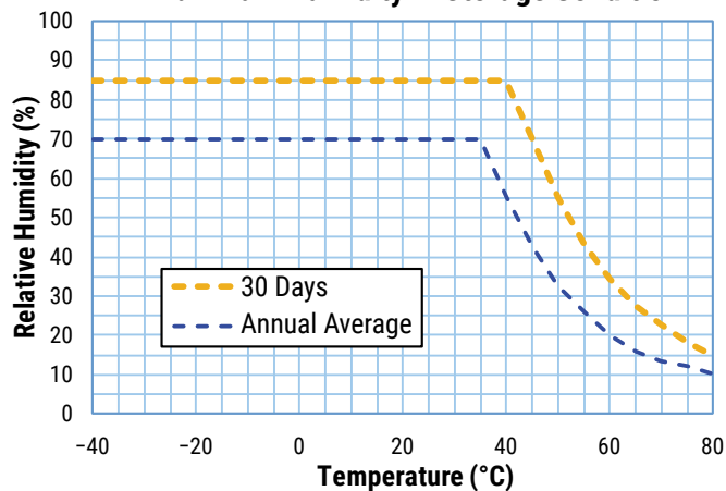
Maximum Humidity in Storage Condition
