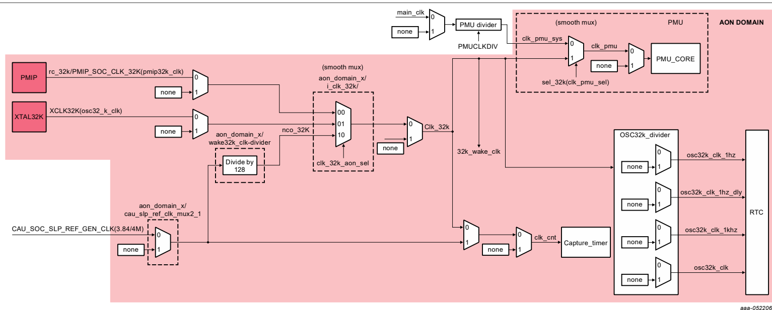
Figure 10. Clock generation - AON domain
