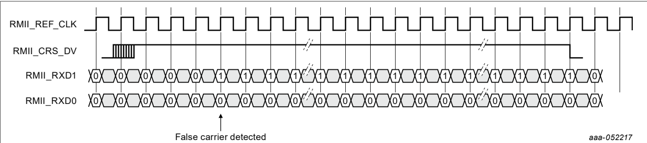
Figure 19. RMII receive operation with false carrier
