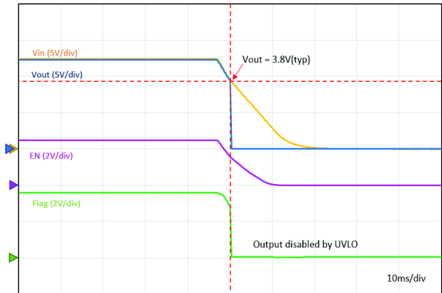
Figure 7. UVLO
